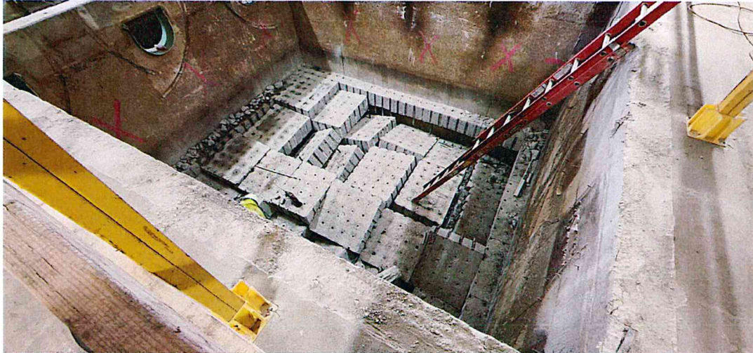
Excavation completed and demo work started for new CCT Transfer Box
