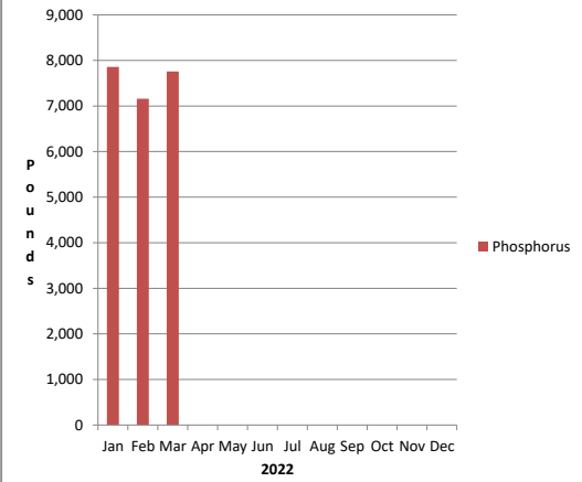
Influent Phosphorus Total Pounds/Mo.
