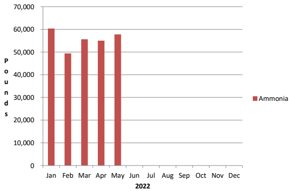
Influent Ammonia Total Pounds/Mo.
